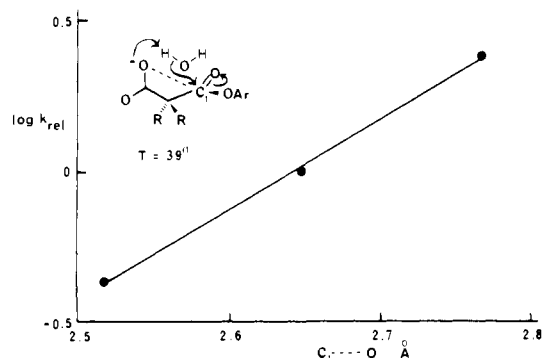
Figure 2. Plot of \log k_{rel} vs. (minimum) C_1 \cdots O distance for a series of monoaryl malonates. Data from ref 6. In this case the crystallographic data are for the parent malonic acids, since the structures for the half esters are not available.
