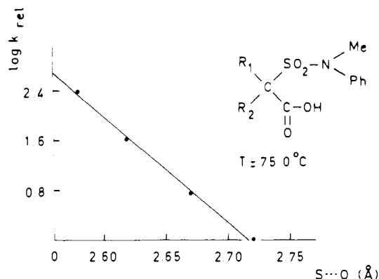
Figure 1. Plot of \log k_{rel} vs. S \cdots O_1 interatomic distance (data from Table II).
